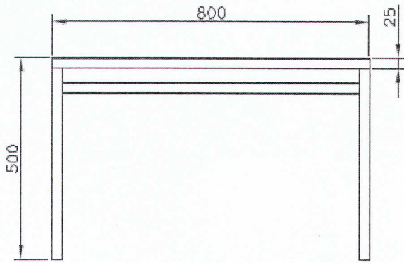
VISTA FRONTAL
