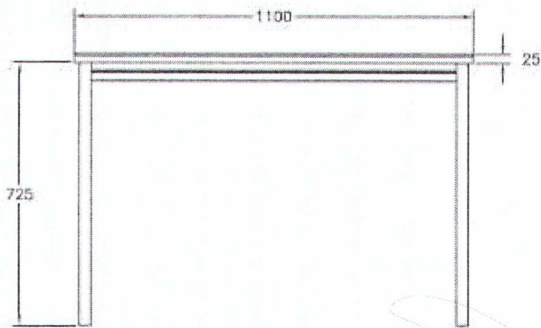
VISTA FRONTAL
