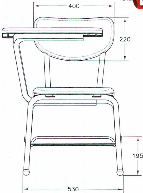
VISTA FRONTAL
